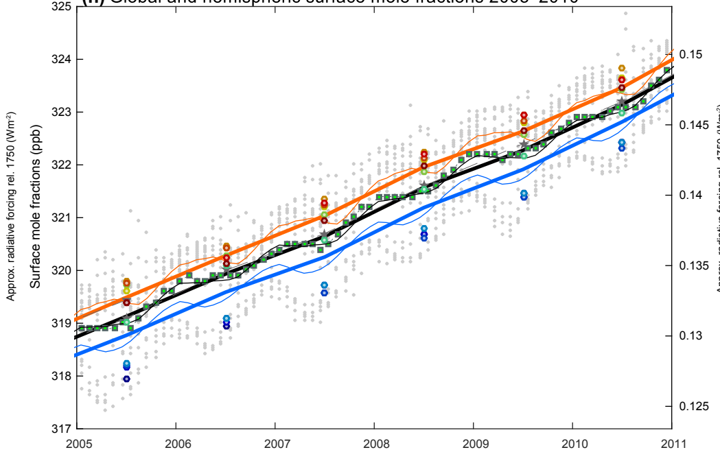
(h) Global and hemispheric surface mole fractions 2005–2010
