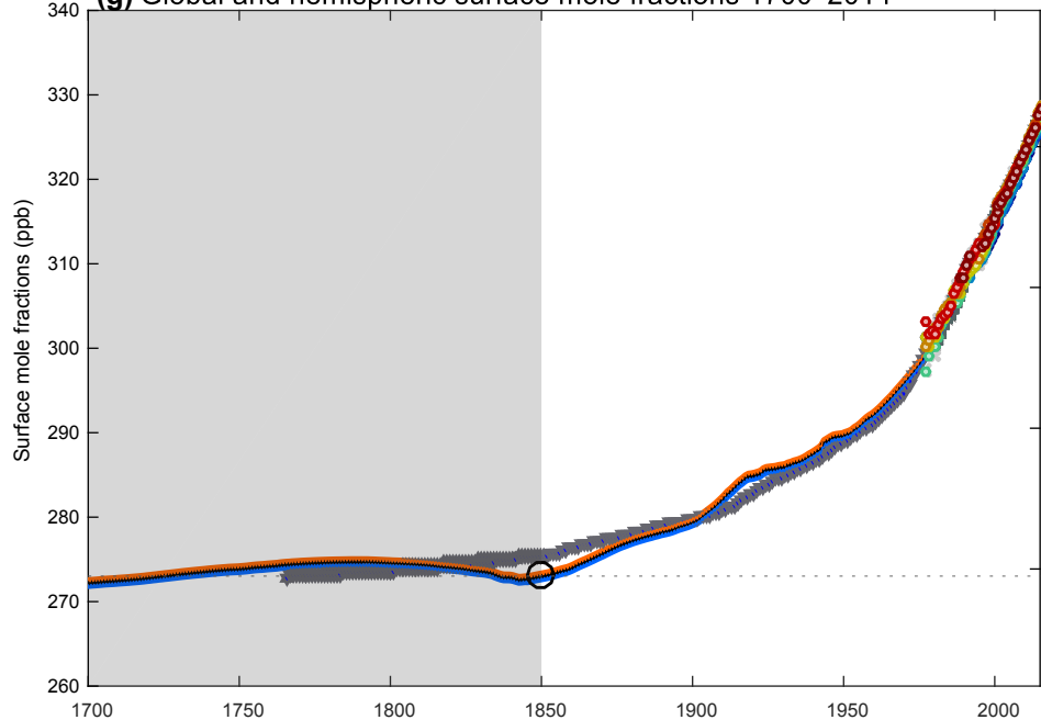
(g) Global and hemispheric surface mole fractions 1700–2014
