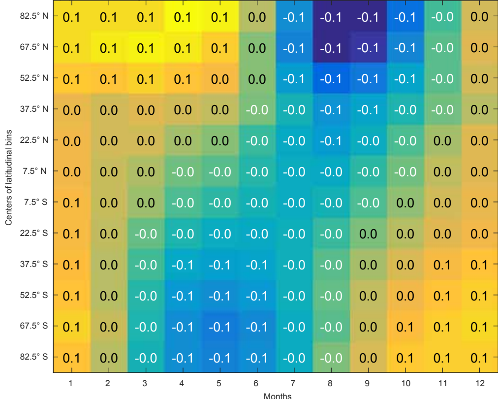
(e) Monthly surface mole fraction field (ppb)
