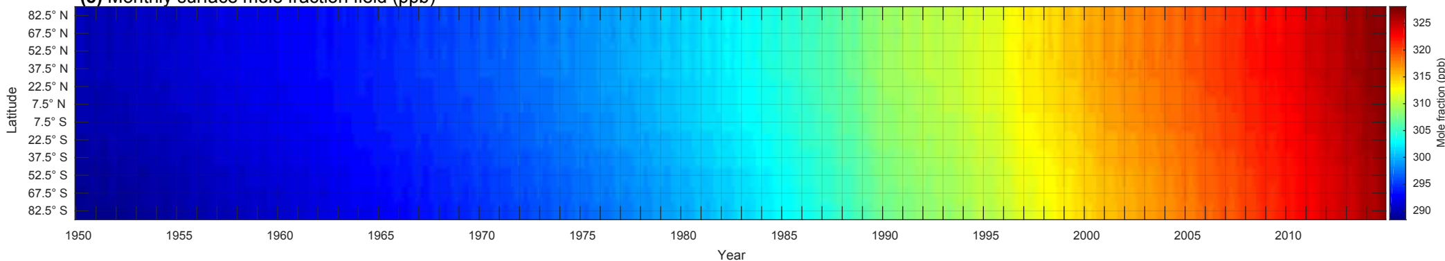
(f) Global and hemispheric surface mole fractions 1950–2014
